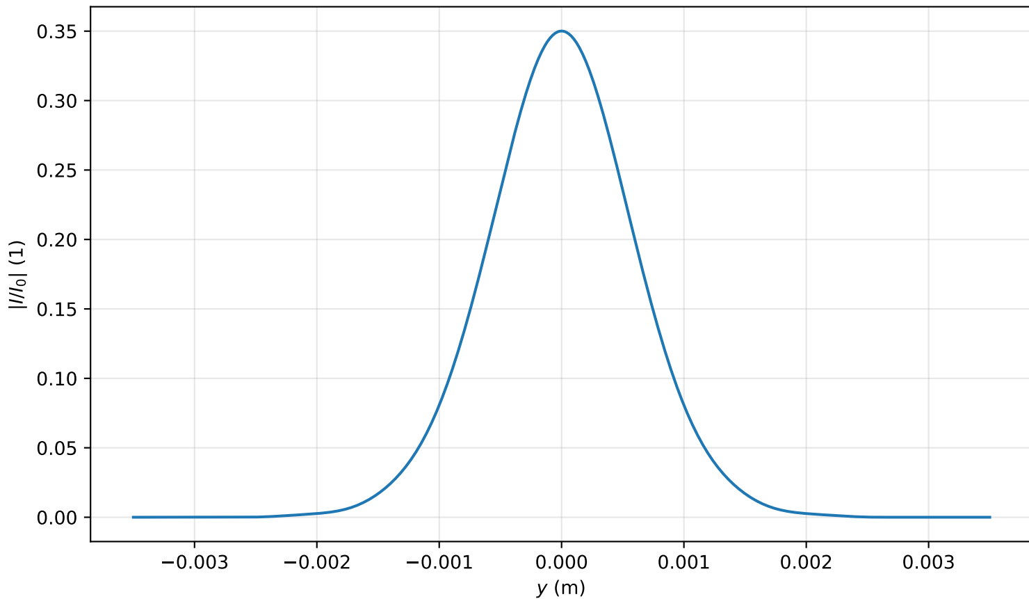
Intensity profile I(x=0, y, z=3.821)/I_0 , P_{in}=0.4P_{cr} , artificial time
